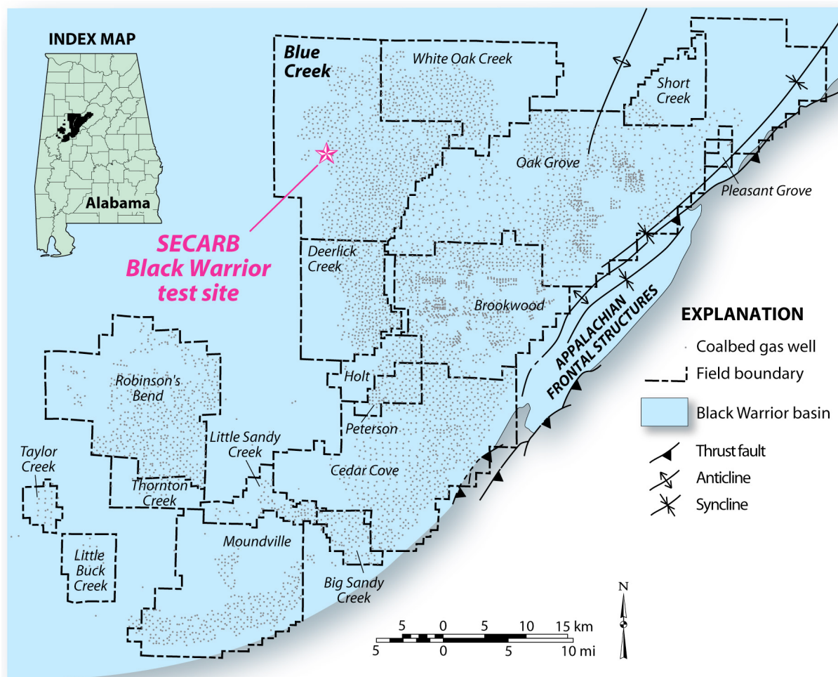
Figure 1. Coalbed methane fields of the Black Warrior Basin in Alabama and location of SECARB Black Warrior Basin Coal Seam Field Test Site
