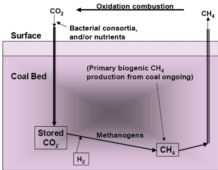
Figure 2. Enhanced CBM followed by microbial regeneration of the CBM reservoir.
