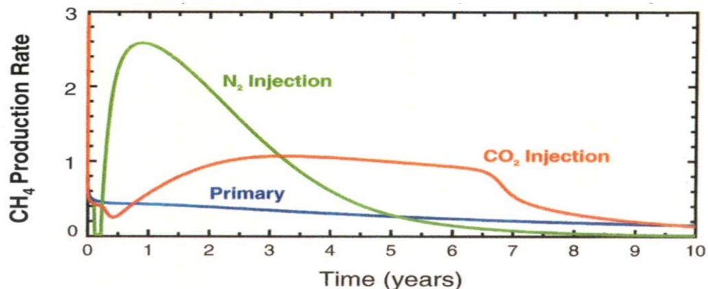
Figure 1. Primary, nitrogen and carbon dioxide injection scenarios for enhanced coalbed methane recovery at Fenn-Big Valley. Injection is at constant flow rate. Production rate is normalized.
